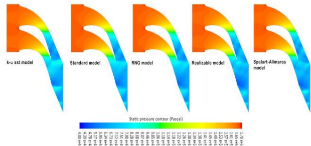
Fig. 6 Comparison of static pressure contours in the passage between blades for different turbulence models P_{t1}=1.689 \text{ bar}, T_0=107.556 \text{ }^\circ\text{C}, P_{t2}=0.650 \text{ bar}.
