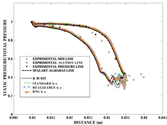
Fig. 4 Comparison between simulation and experimental results for pressure ratio on pressure and suction surfaces P_{t1}=1.689 \text{ bar}, T_0=107.556 \text{ }^\circ\text{C}, P_{t2}=0.650 \text{ bar}.
