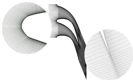
Fig. 2 Structured mesh arrangement
