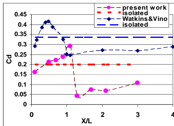
Fig. 15 Variation of vehicle drag coefficients trend compared to previous studies
