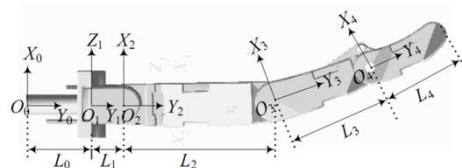
Fig. 2 Cartesian coordinate system in the thumb model
