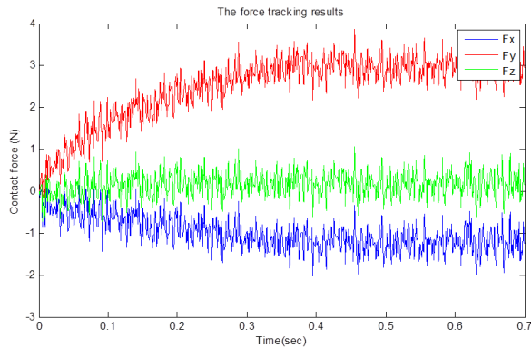
Fig. 9 Thumb force tracking
