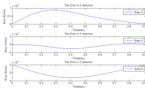
Fig. 19 Tracking error of Exoskeleton in Desecration coordinate
