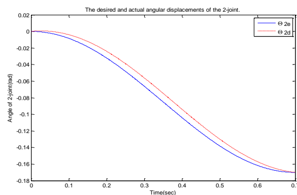
Fig. 7 Desired and actual angular displacements of the joint 2
