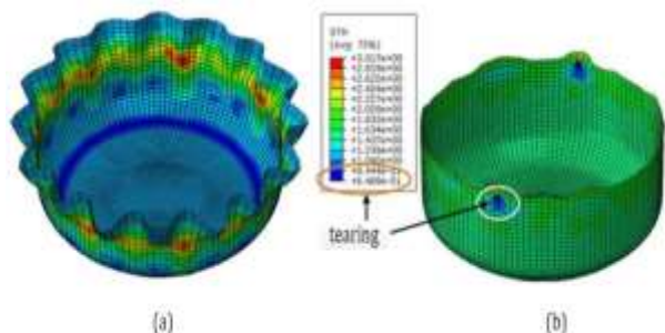
Fig. 4 (a): Wrinkling observed in the first step of the process without applying the blank holder force; and (b): tearing of the sheet.
