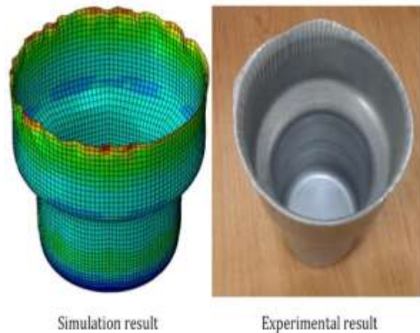
Fig. 14 The sheet wall wrinkling as a result of low amount of blank holder force.
